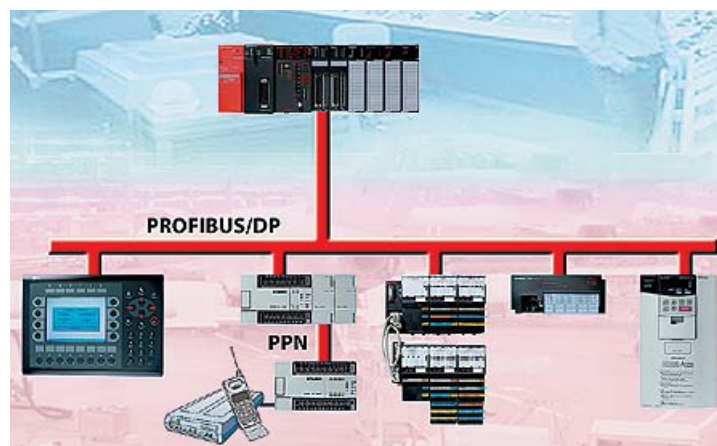
Example of frequency inverter network connection via a Profibus/DP interface
