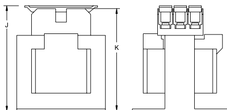
Transformer with Fuse Holder and Covers
