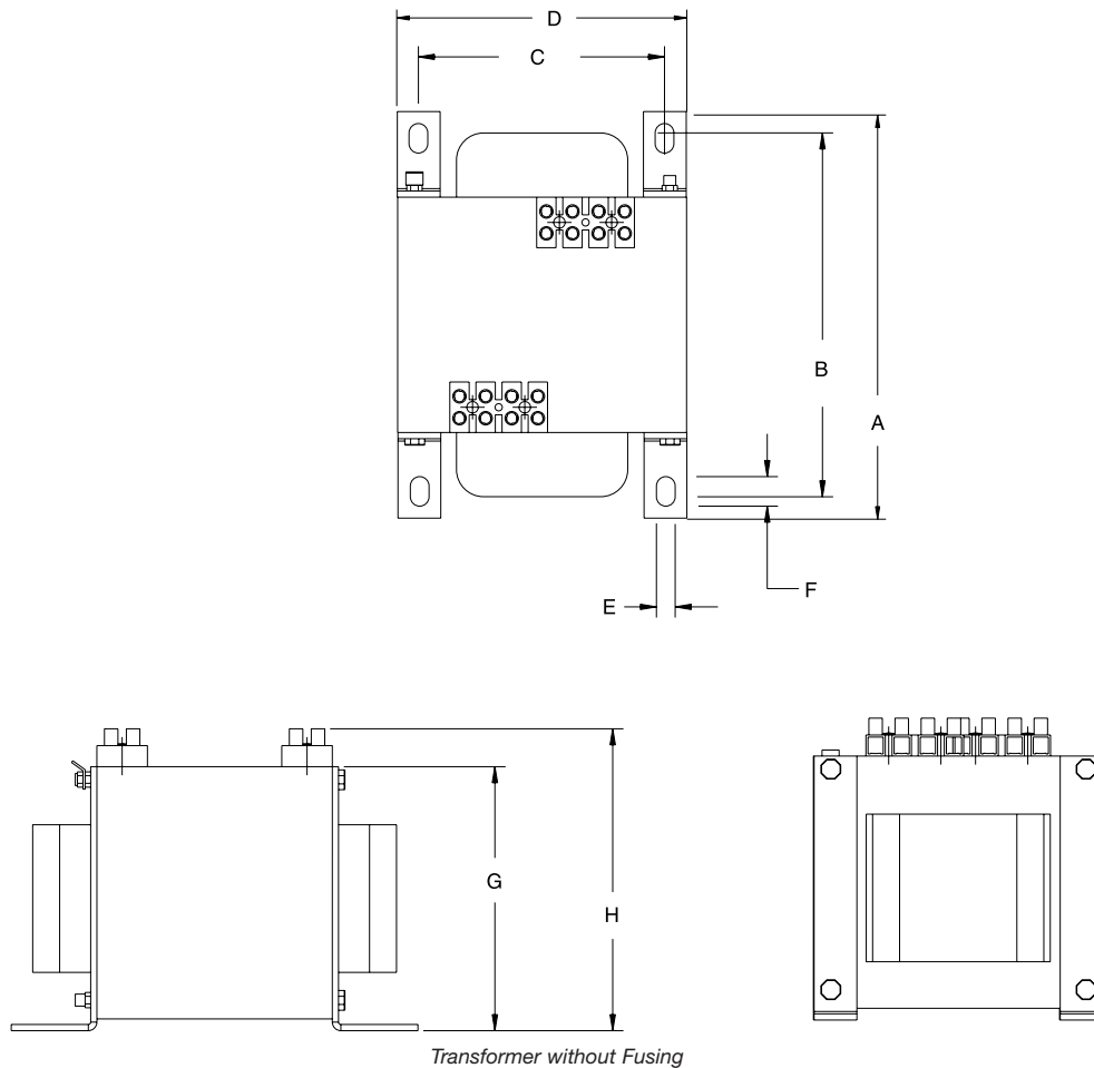
Transformer without Fusing
