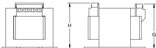
Transformer without Fusing
